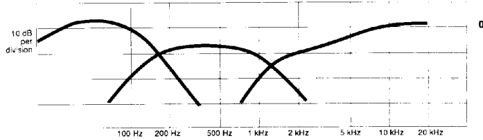
Recommended cross-over setting for DTH Sub and DTH 1 Triamp mode.
